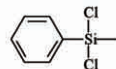
Methylphenyldichlorosilane
