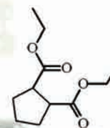
Diethyl-1,2-cyclopentane-dicarboxylate
