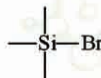
Trimethylphenylsilane
